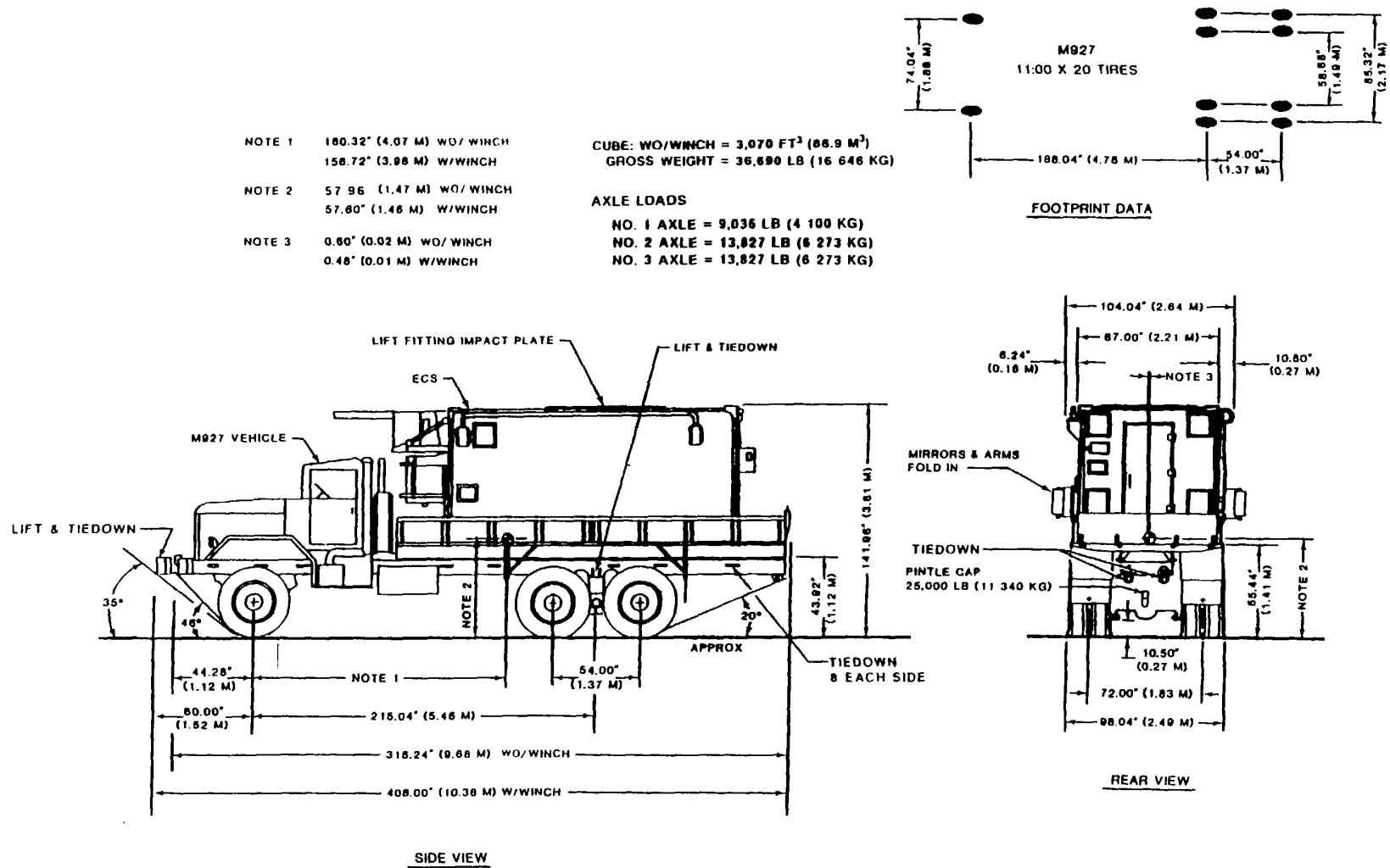
Figure 2-6. Engagement control station on an M927
