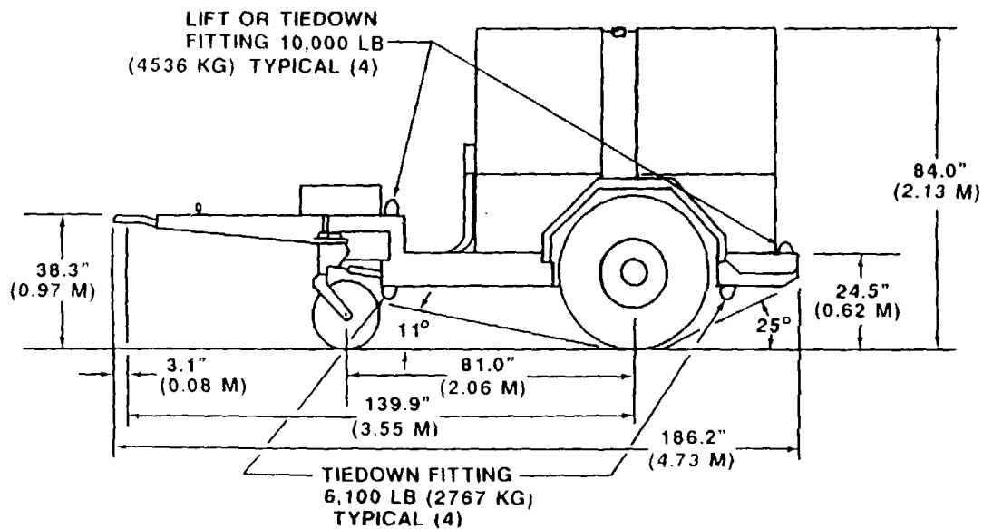
Figure 2-25. Electrical power unit (EPU II) PU-789/M, trailer-mounted
