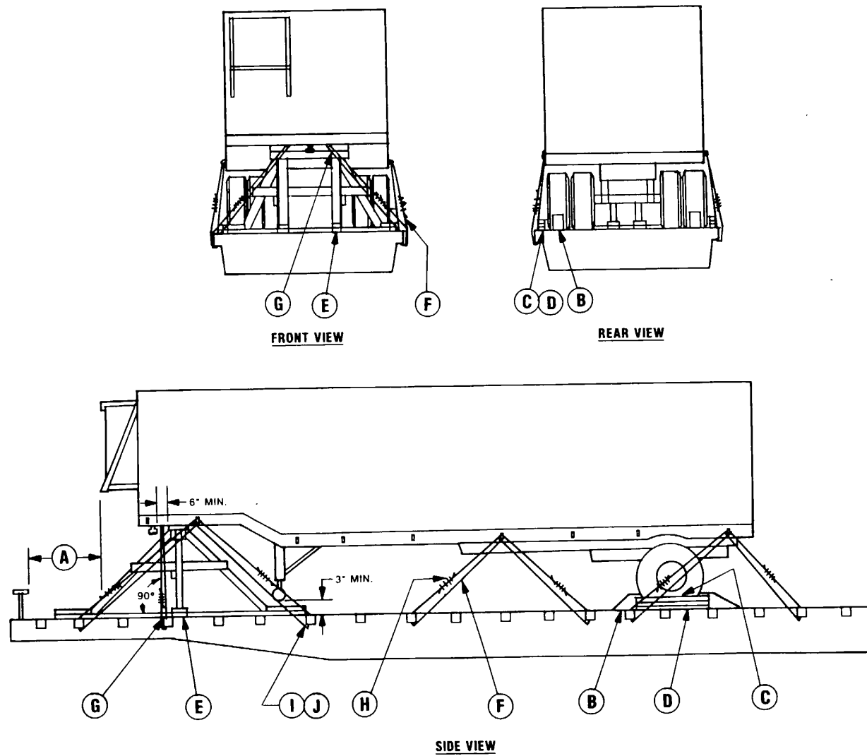
Figure 7-4. Blocking and tiedown of the PATRIOT system van-type semitrailer-mounted components on CONTUS general-purpose faltcars.
