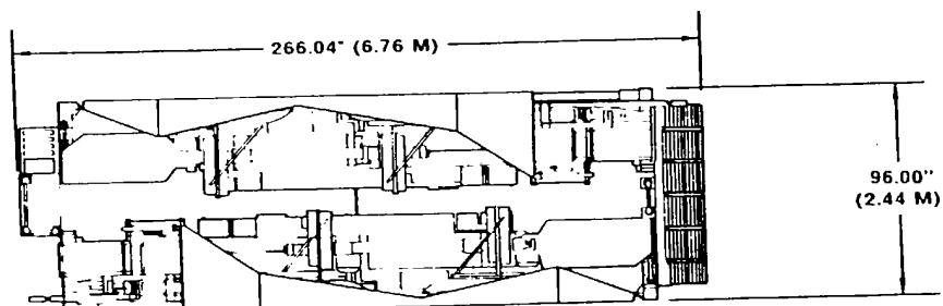
ANTENNA MAST GROUP GUIDED MISSILE, OFF-LOADED PLAN VIEW
