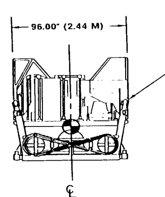
ANTENNA MAST GROUP GUIDED MISSILE, OFF-LOADED END VIEW
