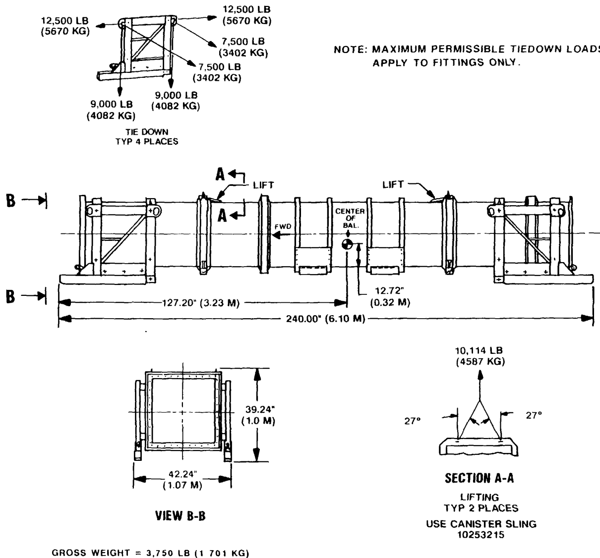
Figure 2-26. Side and end views of missile round (MR) canister.
