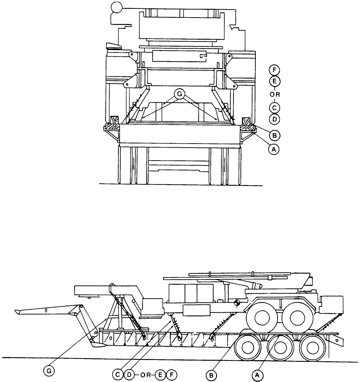
Figure 5-5. Side and rear views of blocking and tiedown of th M860A1 semitrailer on an M870 semitrailer.
