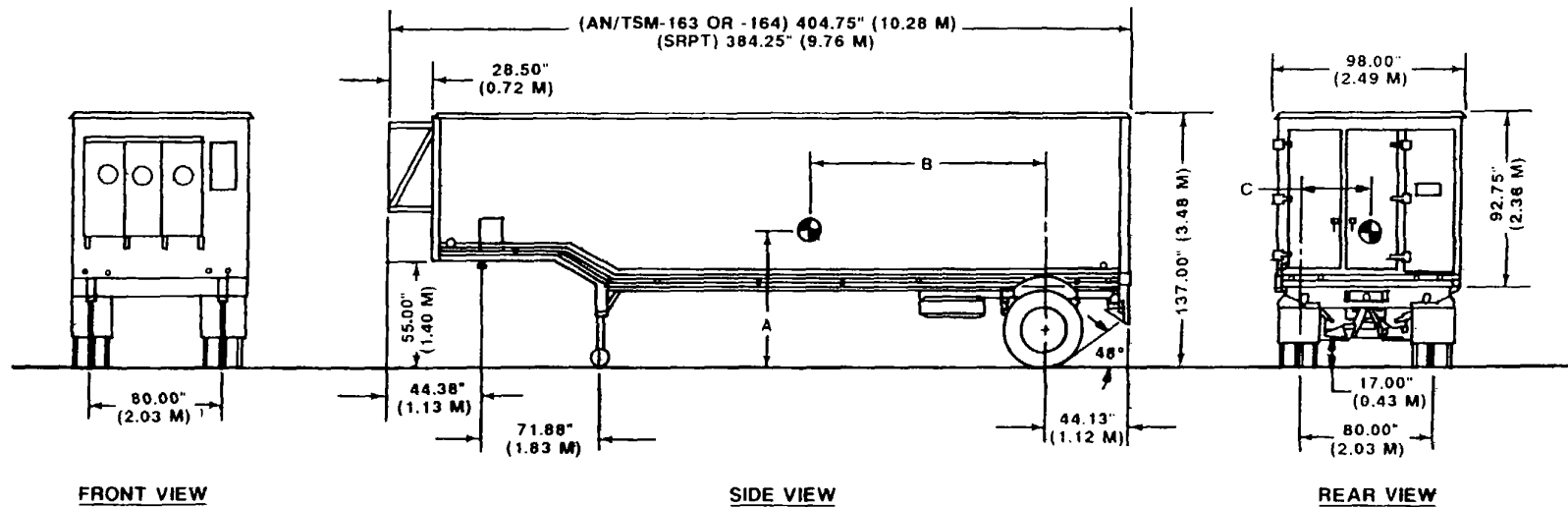
Figure 2-14. Battalion maintenance center AN/TSM-163, or small repair parts transporter M1032, mounted in a modified M373A2 semitrailer van
