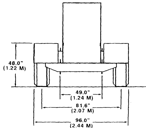
Figure 2-25. Electrical power unit (EPU II) PU-789/M, trailer-mounted
