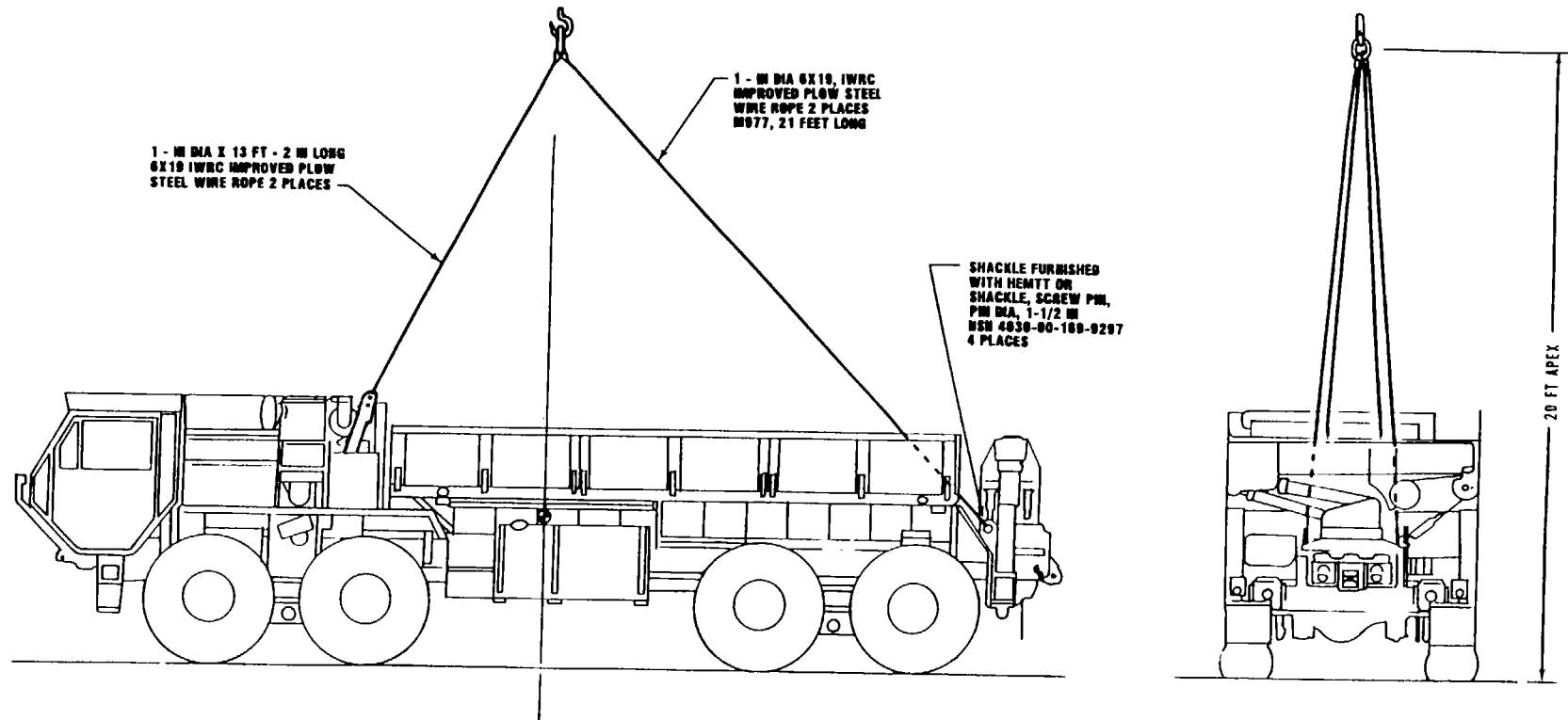
Figure 6-1. Typical lifting diagram for the M977.
