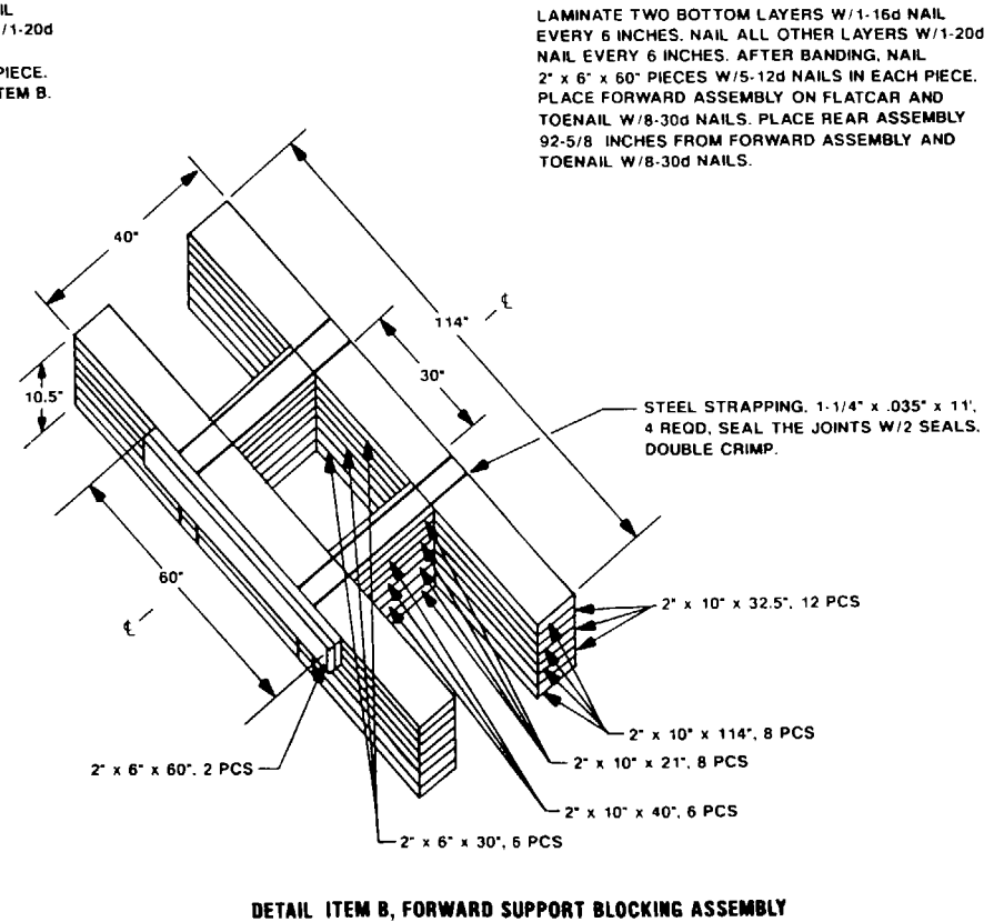
Figure 7-10. RS special blocking detail.
