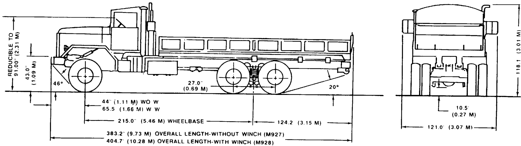
Figure 2-19. M927, 5-ton, 6 x 6 truck.
