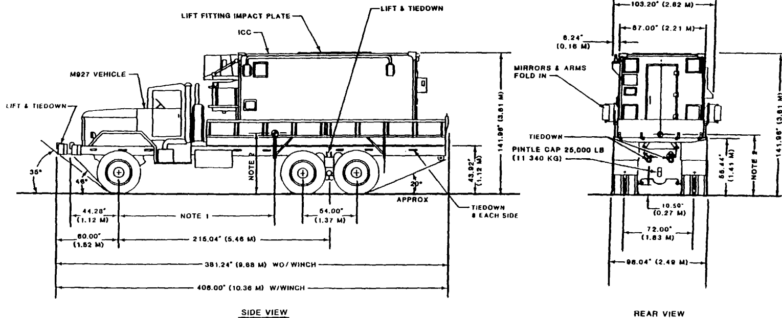
Figure 2-7. Information and coordination central mounted on an M927 2-10
