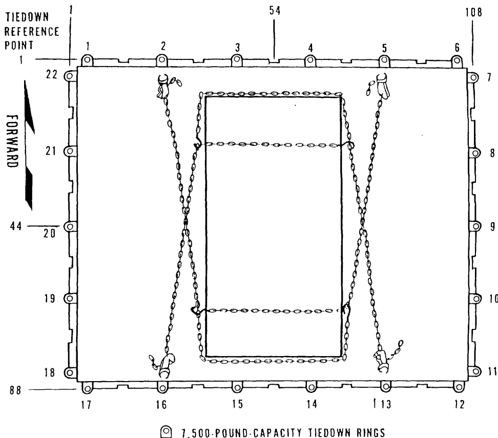
Figure 4-15. LS electrical power unit secured to one HCU-6/E pallet
