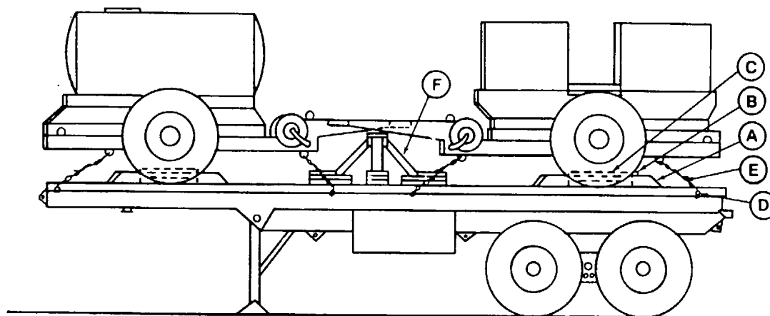
Figure 5-7. Blocking and tiedown of the PATRIOT trailers on an M127A1 semitrailer.
