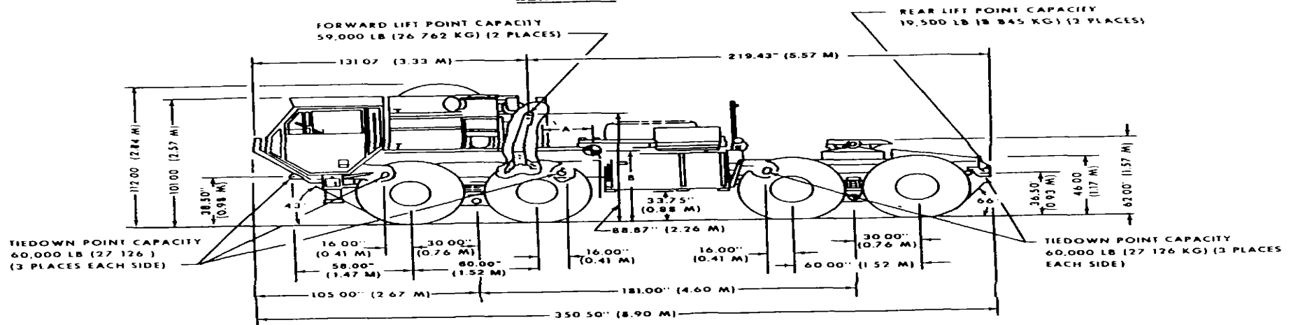
LEFT-SIDE VIEW
