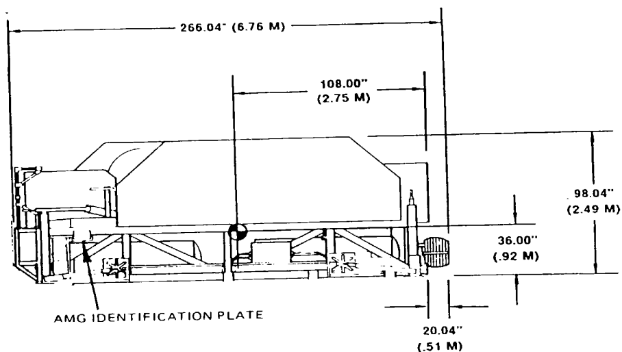
ANTENNA MAST GROUP GUIDED MISSILE, OFF-LOADED SIDE VIEW
