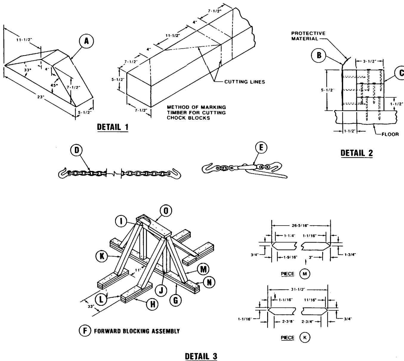
Figure 5-8. Blocking and tiedown details for the PATRIOT trailers.
