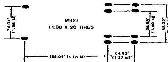
FOOTPRINT DATA
