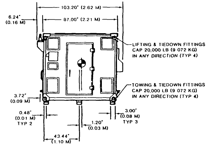
REAR VIEW
