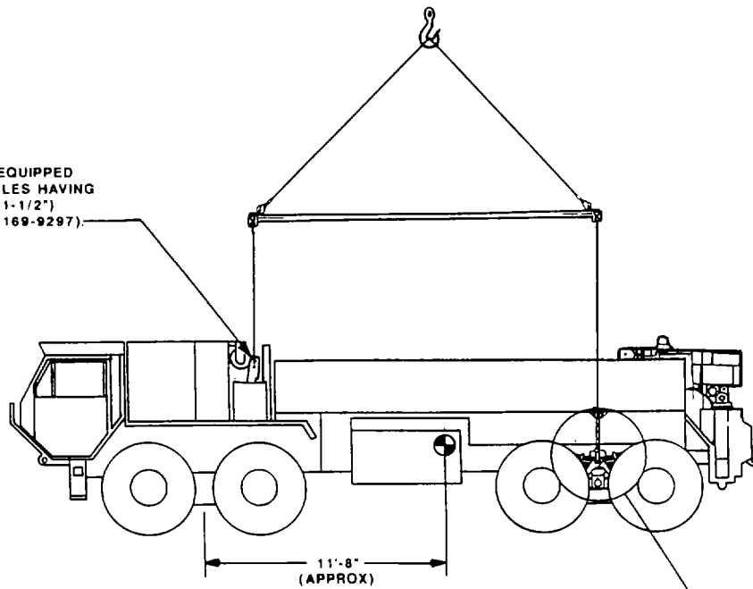
ELEVATION VIEW
