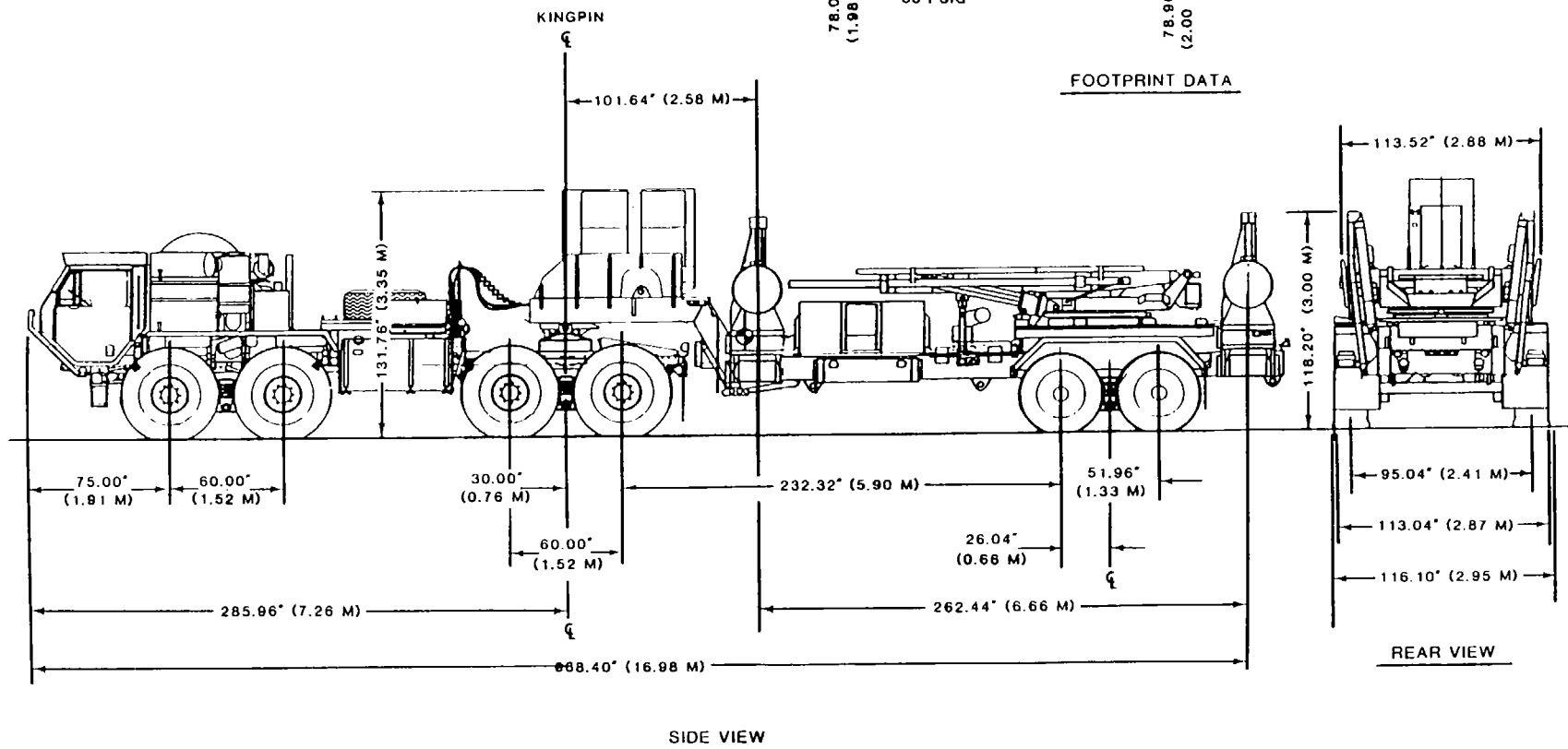
Figure 2-9. Launching station M901, semitrailer-mounted, towed by an M983 truck-trailer 2-13
