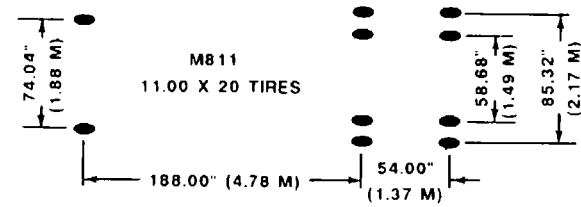
FOOTPRINT DATA
